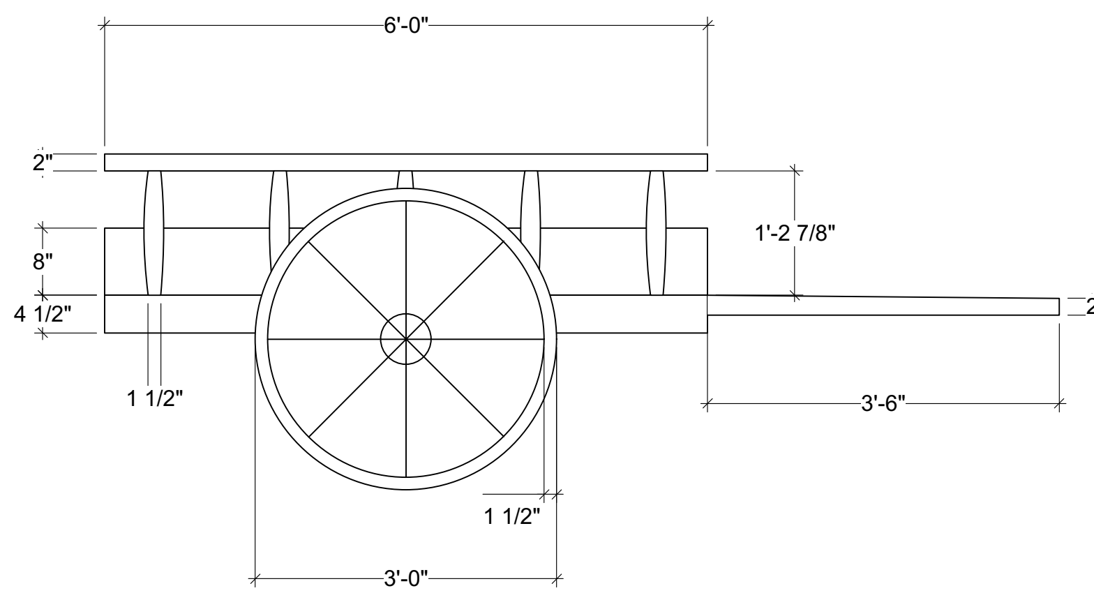
Cart Side View Scale: 3/4" = 1'0"
