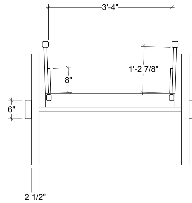
Cart Front View Scale: 3/4" = 1'0"
