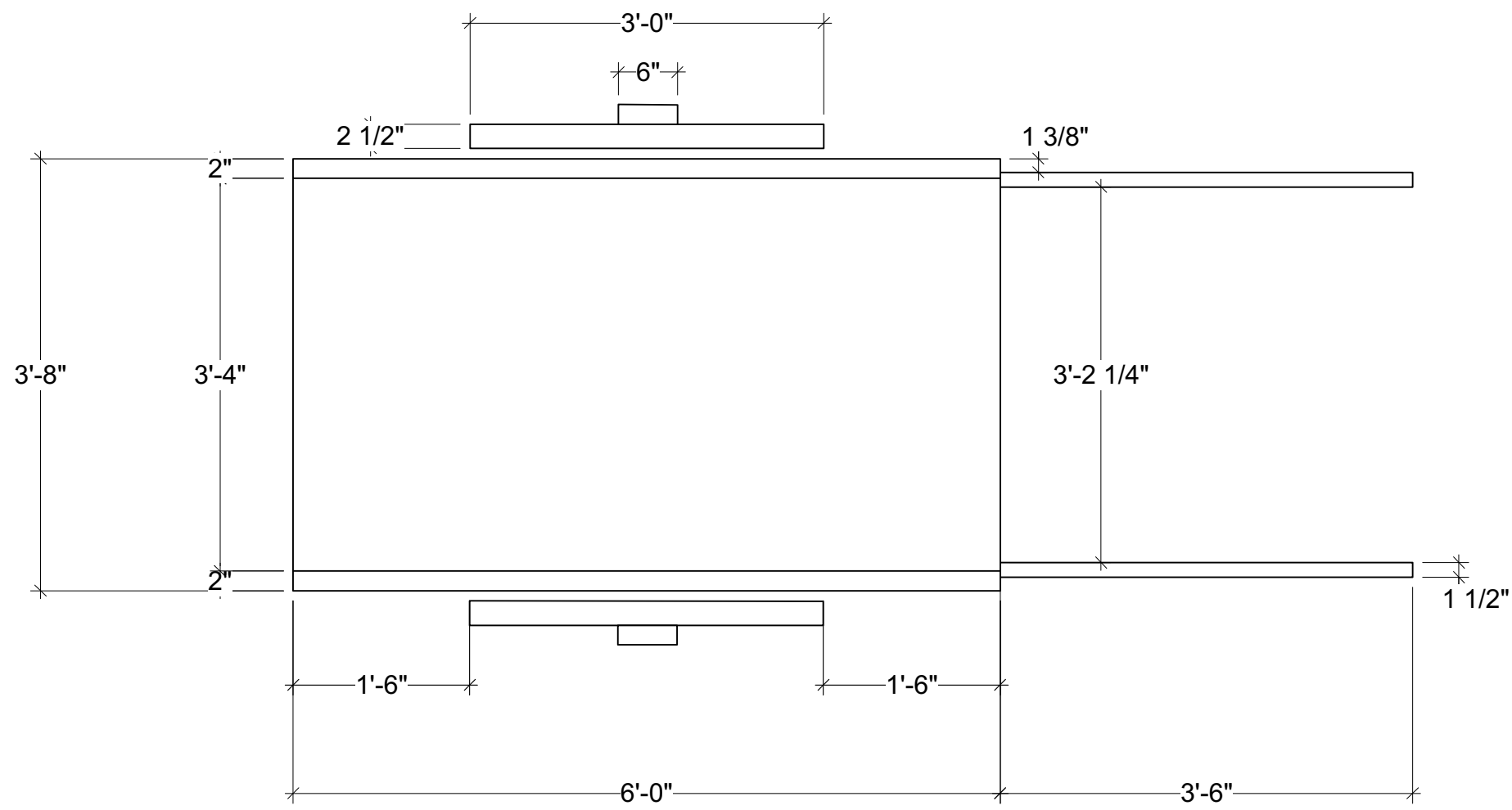
Cart Plan View Scale: 3/4" = 1'0"
