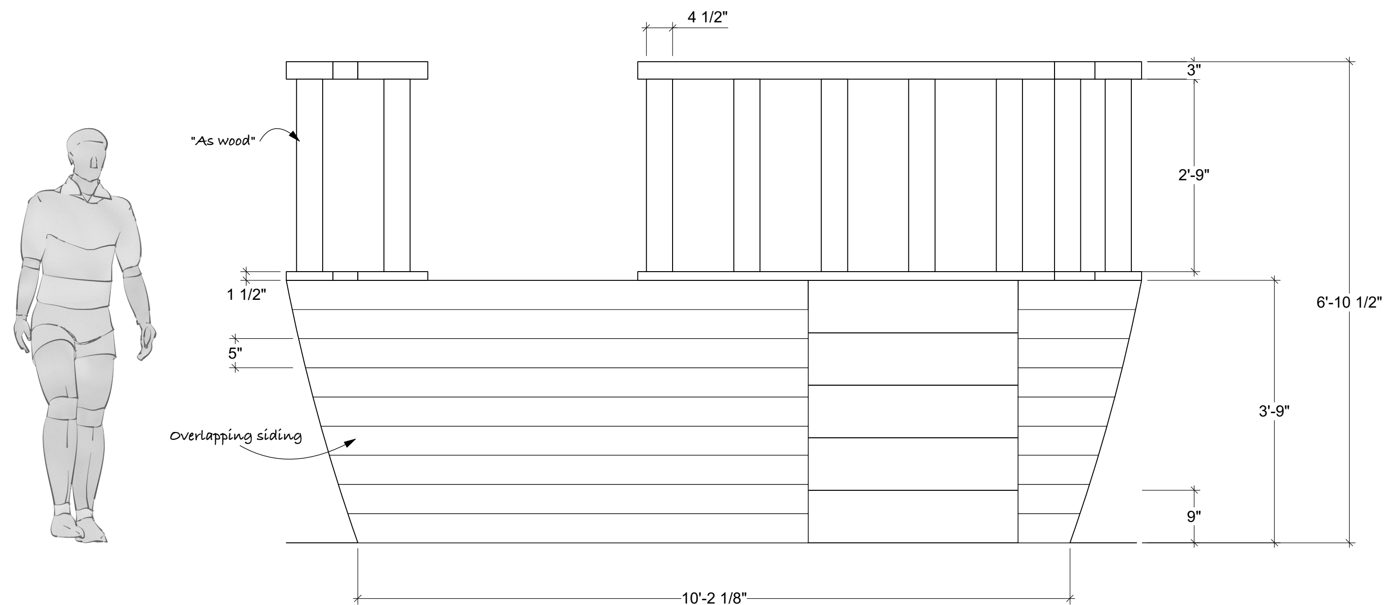
Ship Front View
