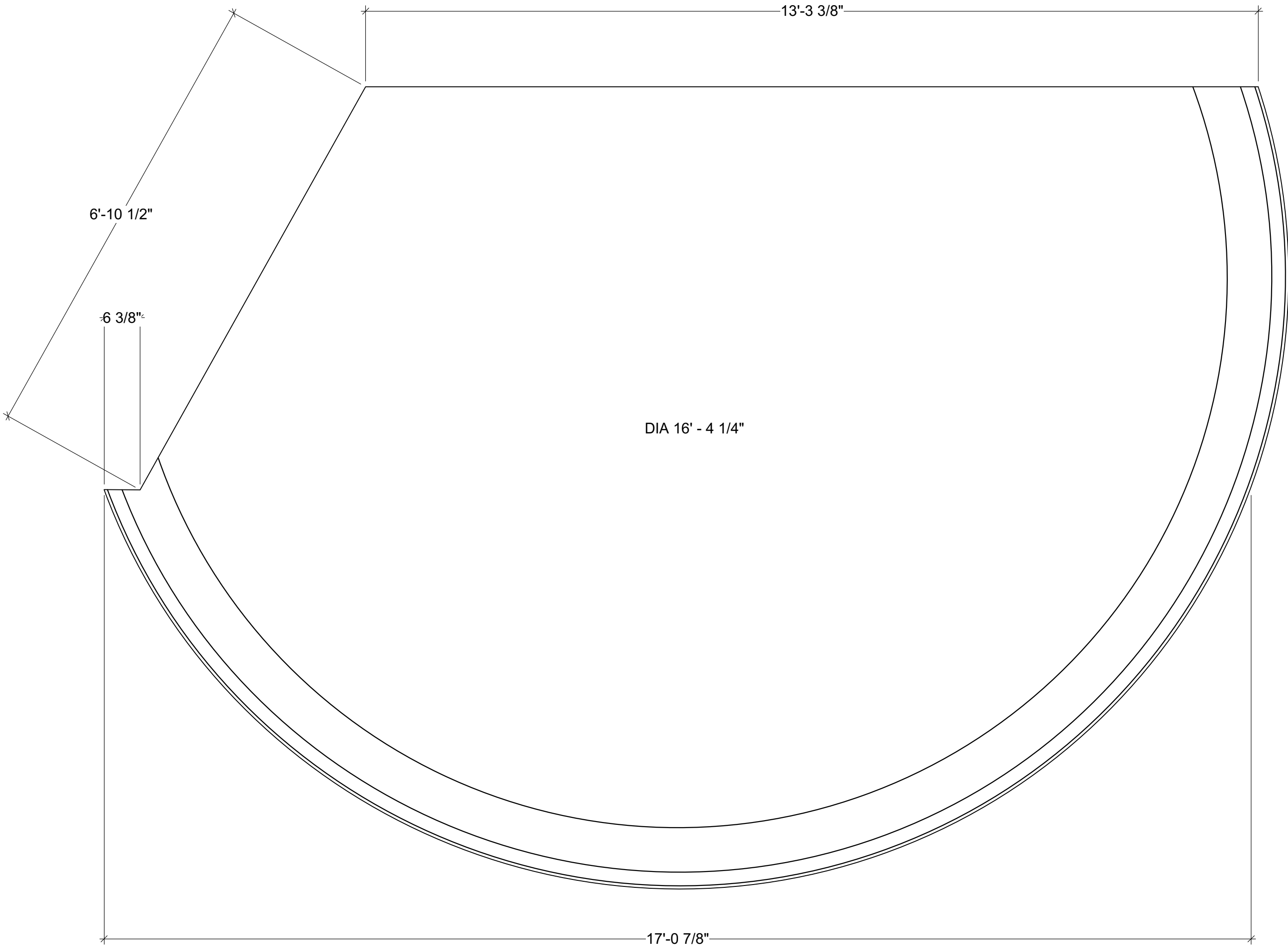
DSR PLAT PLAN VIEW
